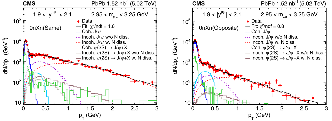
FIG. 5. The corrected transverse momentum spectra of \mu^+\mu^- pairs with a dimuon invariant mass in the J/\psi mass window of ( 2.95 < m_{\mu^+\mu^-} < 3.25 GeV) in “0nXn(Same)” (left) and “0nXn(Opposite)” (right) events. The results of the fit are shown by the various curves. The vertical bars on the data points represent the statistical uncertainty.
