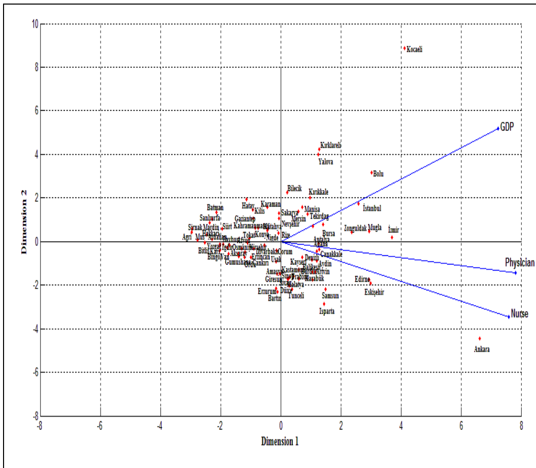
Figure 4: Covariance Biplot
