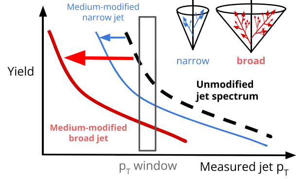
Fig. 1. Schematic diagram of the potential selection bias due to jet energy loss that may occur when selecting jets based on their p_T . Broader structures are expected to be more quenched (thicker red line and arrow), whereas narrower structures are expected to be quenched less (thinner blue line and arrow). Combined with the steeply falling jet p_T spectrum, this can lead to a preferential selection of narrow jets in a given jet p_T interval, as indicated by the vertical rectangular box. The dashed curve represents the jet p_T spectrum in the absence of medium-induced jet modifications.
