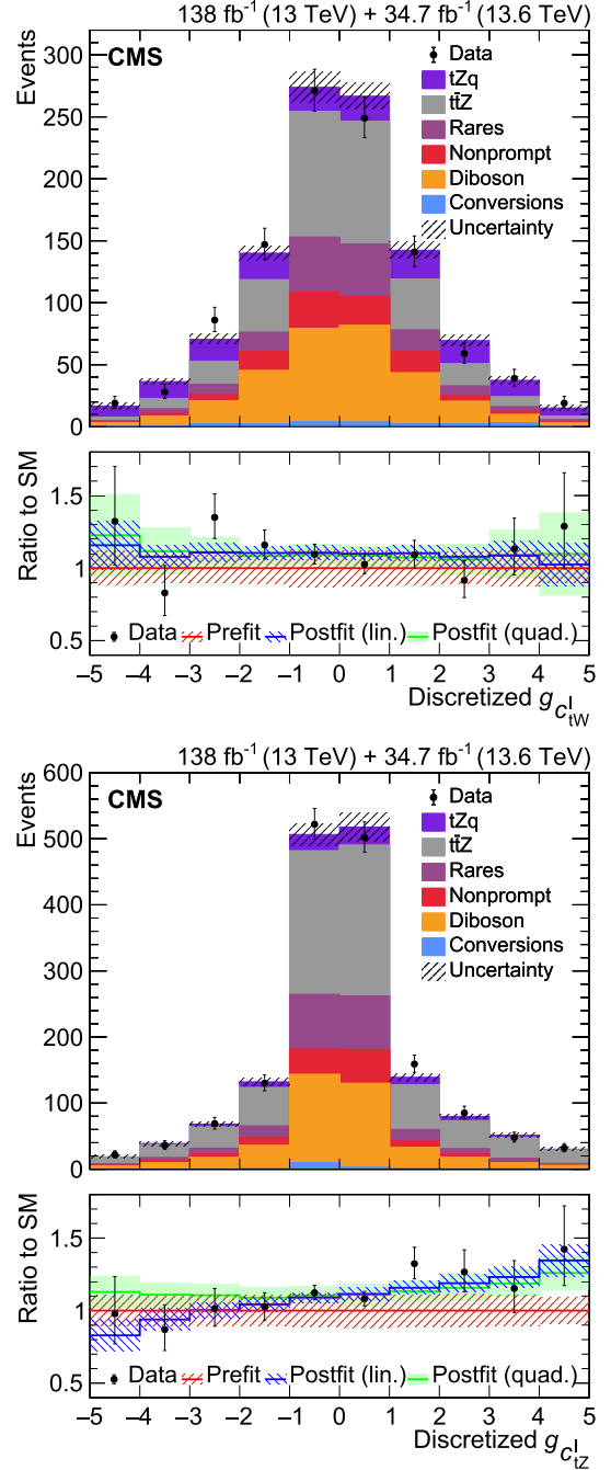
Fig. 3. Upper (lower): Distribution of the discretized g_{c_{tW}^I} ( g_{c_{tZ}^I} ) for events in the c_{tW}^I -like ( c_{tZ}^I -like) category, compared with the predictions obtained when all fit parameters are set to their maximum likelihood value in the linear fit, where c_{tW}^I and c_{tZ}^I are determined simultaneously. The lower panels show the ratio between data (black dots), the prediction of the linear (blue line), and quadratic (green line) fits, over the prefit value. The red, blue, and green bands show the prefit uncertainty and the postfit uncertainties of the linear and quadratic fits, respectively. (For interpretation of the references to colour in this figure legend, the reader is referred to the web version of this article.)
