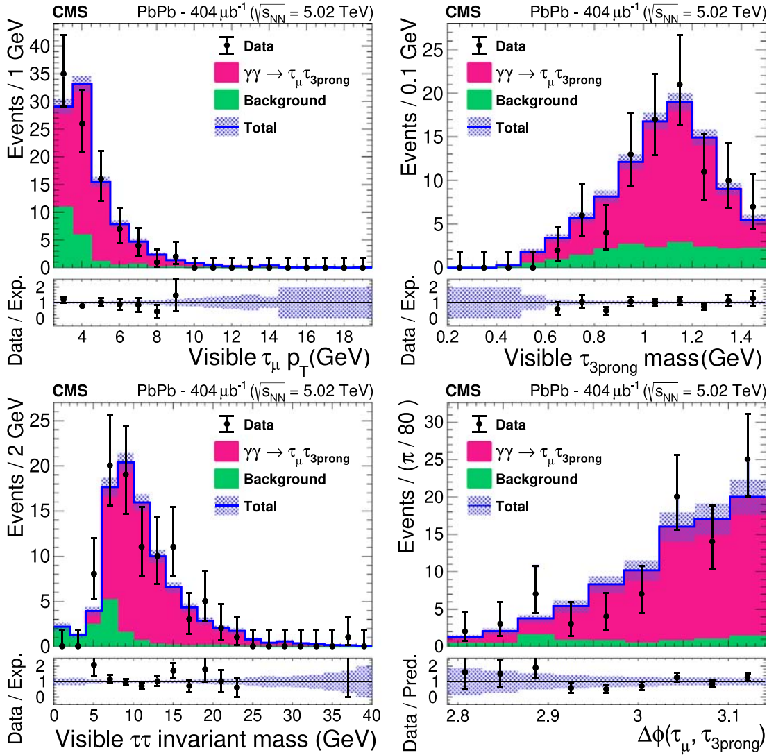
Fig. 108. Transverse momentum of the muon originating from the \tau_\mu candidate (upper left). Invariant mass of the three pions forming the \tau_{3\text{prong}} candidate (upper right). Invariant mass of the \tau^+\tau^- system (lower left). The \Delta\phi(\tau_\mu, \tau_{3\text{prong}}) azimuthal difference (lower right). In all plots, the signal component (magenta histogram) is stacked on top of the background component (green histogram). The sum of signal and background is displayed by a blue line and the shaded area shows the statistical uncertainty. The data are represented with black points and the uncertainty is statistical only. The lower panels show the ratios of data to the signal-plus-background prediction and the shaded bands represent the statistical uncertainty in the prefit expectation.
