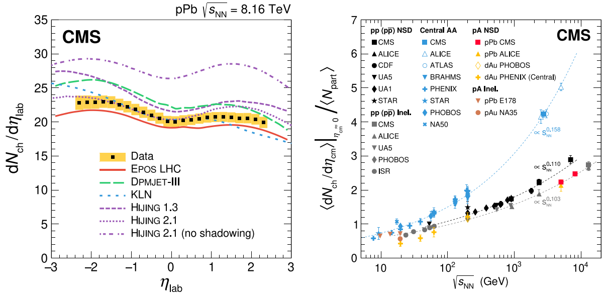
Fig. 85. Left: Pseudorapidity density of charged hadrons in the range |\eta_{lab}| < 2.4 in pPb collisions at 8.16 TeV. The results are compared to predictions from the MC event generators EPOS LHC [123,476] (v3400), HIJING [124] (versions 1.3 [477] and 2.1 [478]), and DPMJET-III [479], as well as from the KLN model [257]. The shaded boxes around the data points indicate their systematic uncertainties. The proton beam goes in the positive \eta_{lab} direction. Right: Comparison of the measured density at midrapidity, scaled by N_{part} in pPb [480,481], pAu [482], dAu [483–485] and central heavy ion collisions [111,234,484,486–497], as well as NSD [235,236,238,239,497–499] and inelastic [234,237,238,500,501] pp collisions. The dashed curves, included to guide the eye, are from Refs. [237,494].
