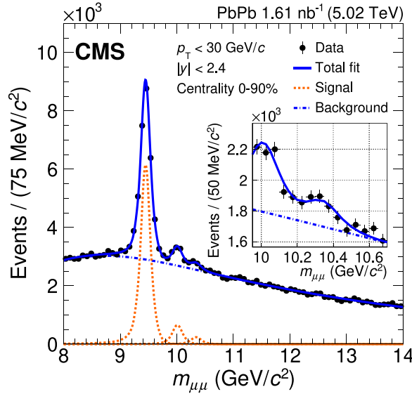
Fig. 81. The dimuon invariant mass distribution measured in PbPb collisions when integrating over the full kinematic range of p_T < 30 GeV and |y| < 2.4 . The solid curves show the fit results, and the orange dashed and blue dash-dotted curves display the three Y states and the background, respectively. The inset shows the region around the Y(3S) meson mass.
