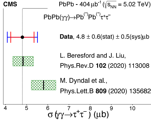
Fig. 109. The \sigma(\gamma\gamma \rightarrow \tau^+\tau^-) cross section, measured in a fiducial phase space region at \sqrt{s_{\text{NN}}} = 5.02 \text{ TeV} . The theoretical predictions [581,582] are computed with leading order accuracy in QED and are represented by the vertical solid lines, which can be compared with the vertical dotted line representing this measurement. The outer blue (inner red) error bars represent the total (statistical) uncertainties, whereas the green hatched bands correspond to the uncertainty in the theoretical predictions, as described in the text. The potential electromagnetic excitation of the outgoing Pb ions is denoted by (^*) .
