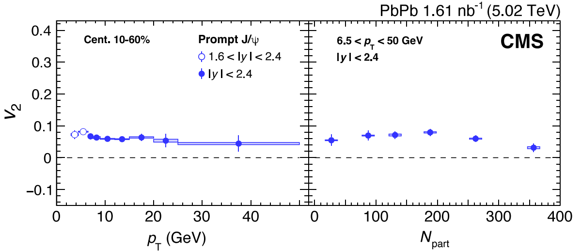
Fig. 84. The prompt J/\psi v_2 as a function of p_T (left) and N_{part} (right), in PbPb collisions at 5.02 TeV. Source: Figure adapted from Ref. [413].
