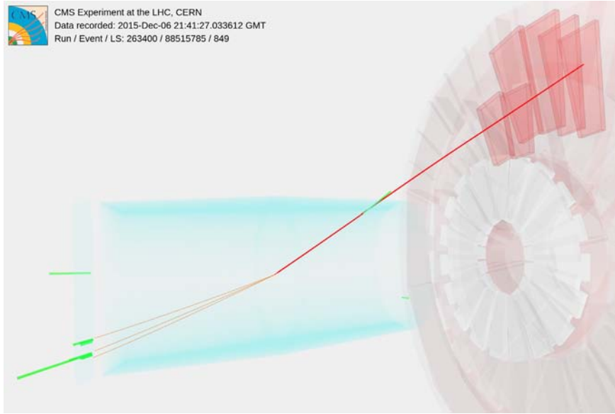
Fig. 101. Event display of a candidate \gamma\gamma \rightarrow \tau^+\tau^- event measured in a PbPb UPC at CMS. The event is reconstructed as corresponding to a leptononic \tau decay (red), \tau \rightarrow \mu^+\nu_\mu\nu_\tau , and a hadronic \tau decay (yellow), \tau \rightarrow \pi^+\pi^-\pi^+\nu_\tau . Source: Figure adapted from Ref. [549].
