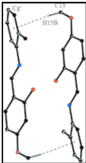
Fig. 2. Part of crystal structure of molecule, showing the C—H... \pi bonds. For clarity, H atoms not included in intermolecular bonding have been omitted. For symmetry codes, see Table 1.
